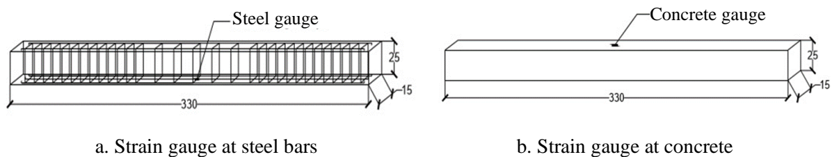
Figure 3 Location of strain gauge
