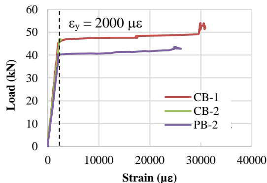
Figure 7 Load-strain of rebars
