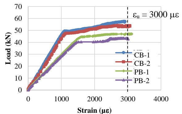
Figure 8 Load-strain of concrete
