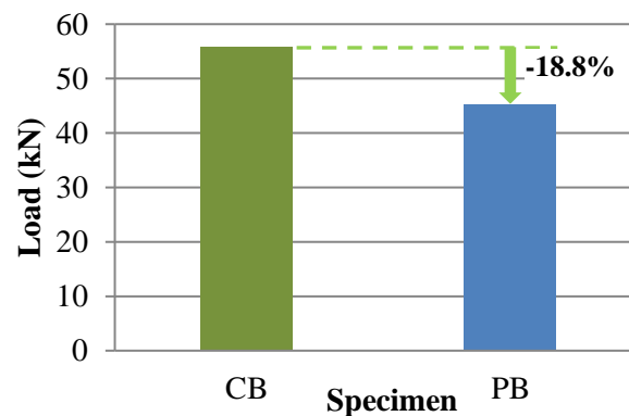
Figure 6 Ultimate capacity
