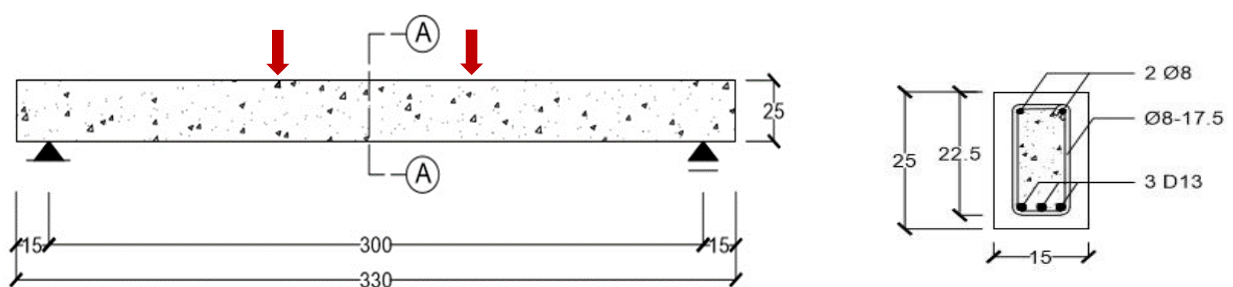
Figure 2 Details of specimens
