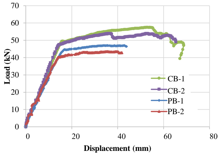
Figure 5 Load-displacement behaviour
