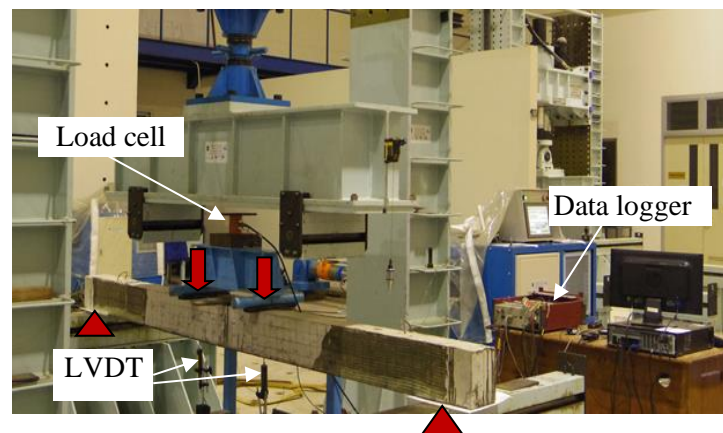
Figure 4 Loading test
