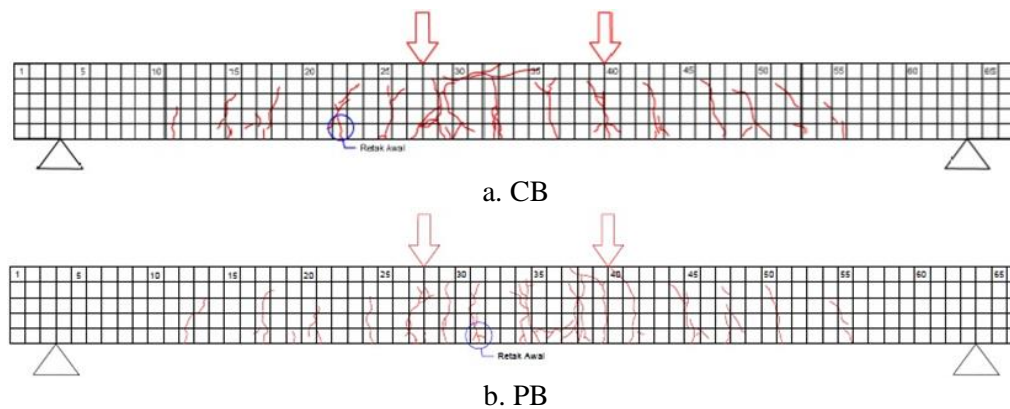
Figure 9 Crack pattern
